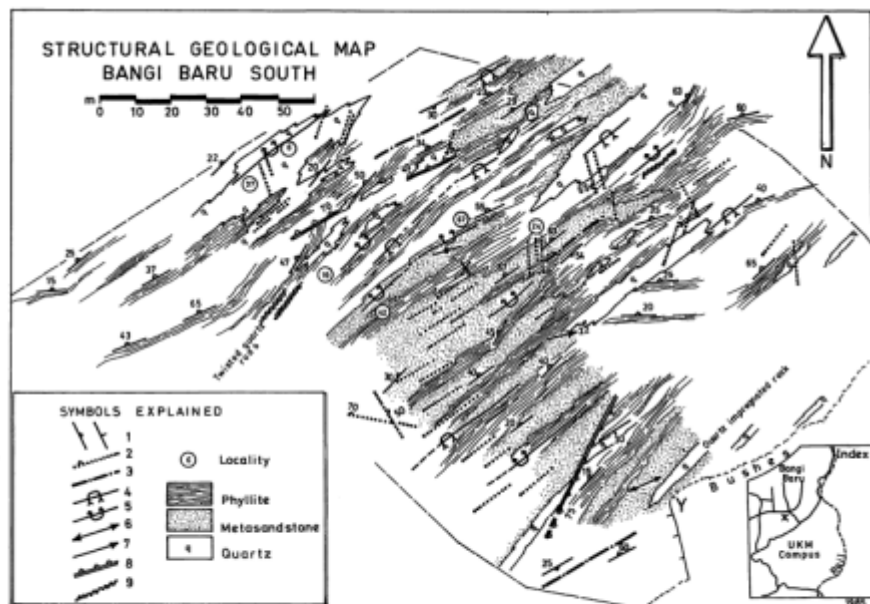
Figure 1 : Structural geology of an area near the roundabout, Bangi Baru (south); inset indicates the locality. Explanation of symbols : 1 = foliation, bedding; 2 = quartz veins (with or without iron oxide); 3 = warp axis determined from foliation patterns on the map; 4 = synform, overturned to isoclinal; 5 = antiform, overturned to isoclinal; 6 = medium fold, horizontal fold axis; 7 = medium fold axis with plunge direction and plunge angle; 8 = fault, triangles indicate dip direction; 9 = twisted, quartz-impregnated fold hinge. The scarp outcrop of figure 9 extends between X and Y. Localities referred to in the text or on other illustrations are indicated on the map.
